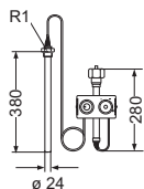
AFT 06
