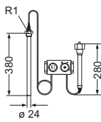
AFT 26
