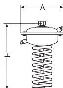
AFD
